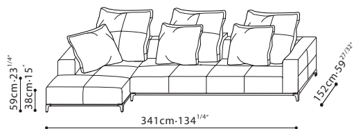
C0130013+C8130002+C8130003+C0130010 +C8130002×2+C8130003×2
